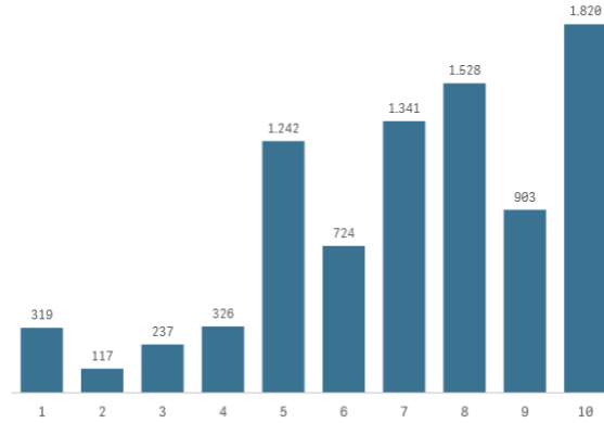
Frequency distribution
